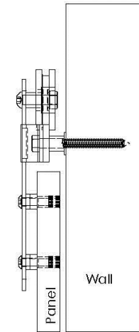
Std Hardware Pack installed with no casing, or other trim
