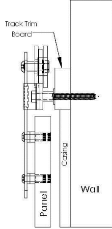
Std Hardware Pack installed on track trim board that is equal to or thicker than casing or other trim
