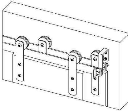
Std Hardware Pack installed with no casing, or other trim
